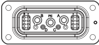
Bottom Connector
