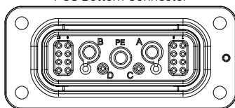
PCS Bottom Connector
